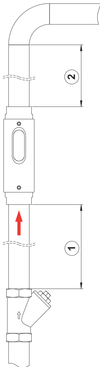
Fig. 7: Strainer
