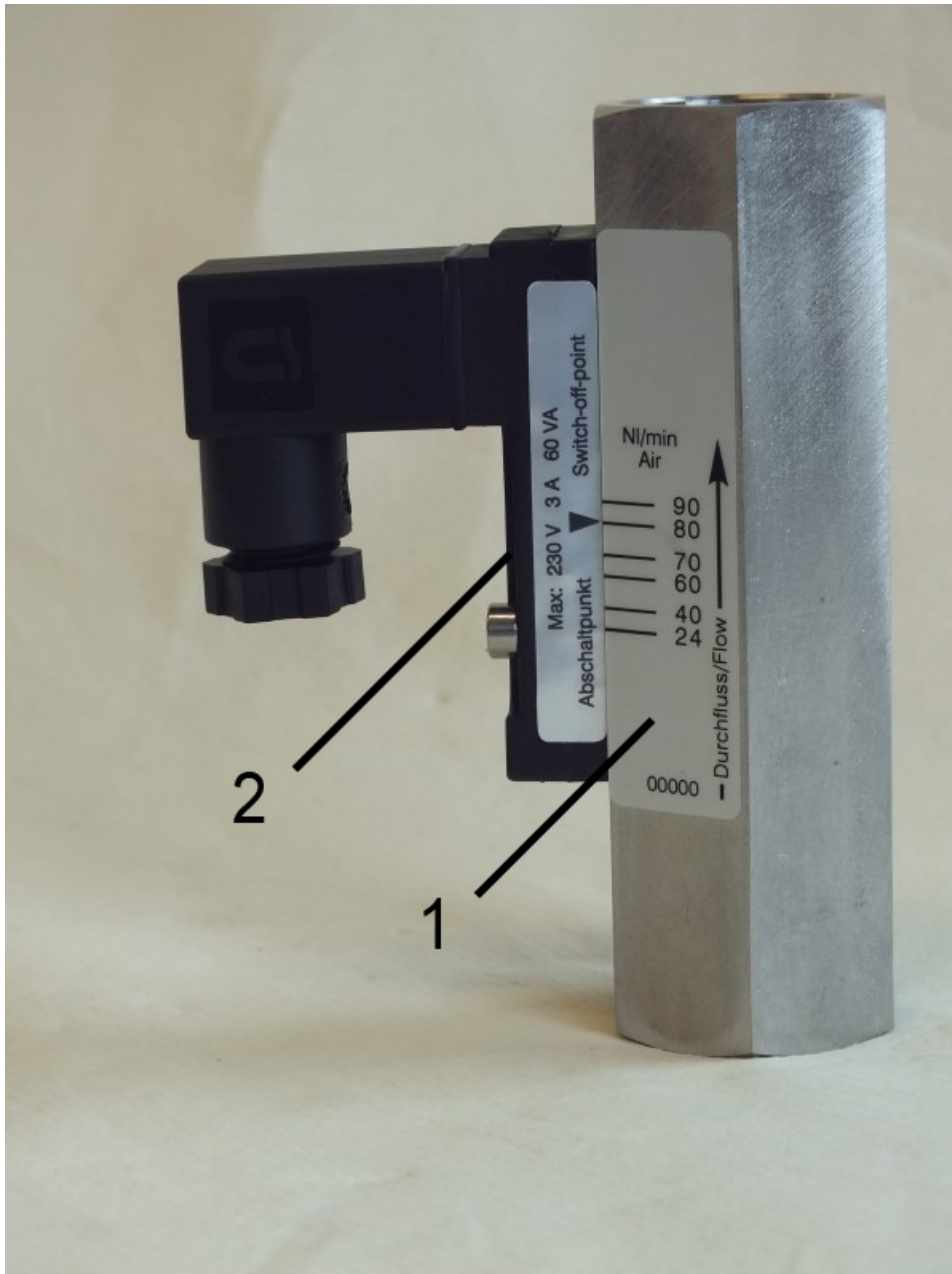
Fig. 1: RVM/U-L2 flow monitor
