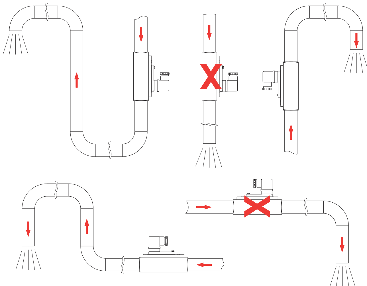
Fig. 7: Unimpeded outlet
