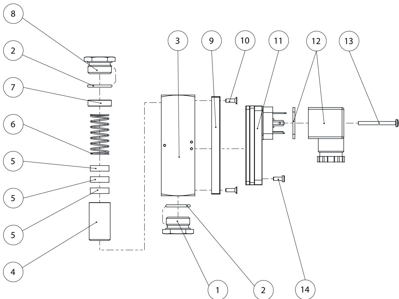
Abb. 57: EZ_RVM_U-L2_SG-30
