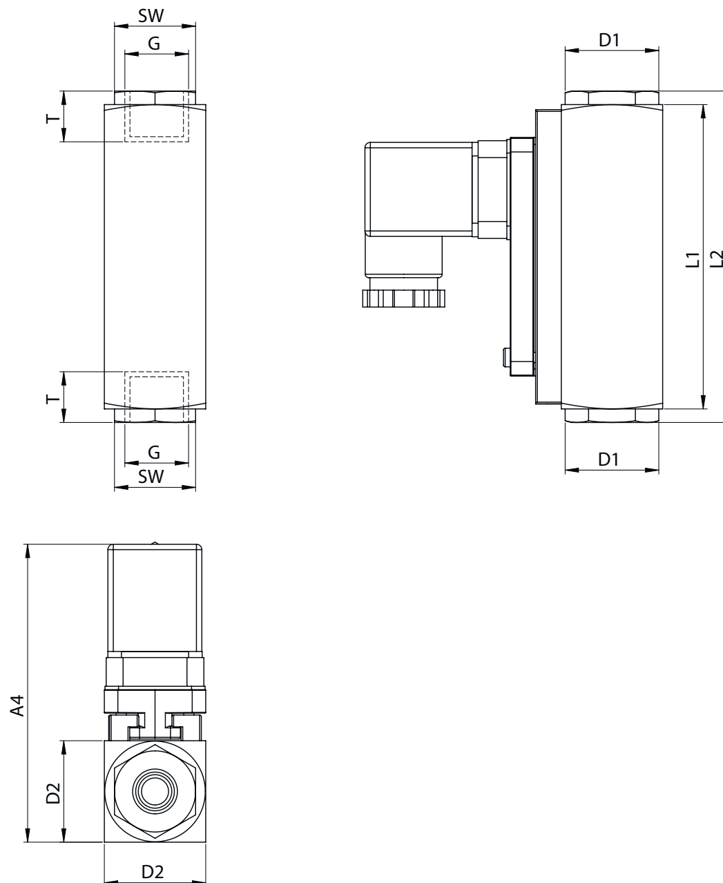
Abb. 56: TZ_RVM_U-L2_SG-30
