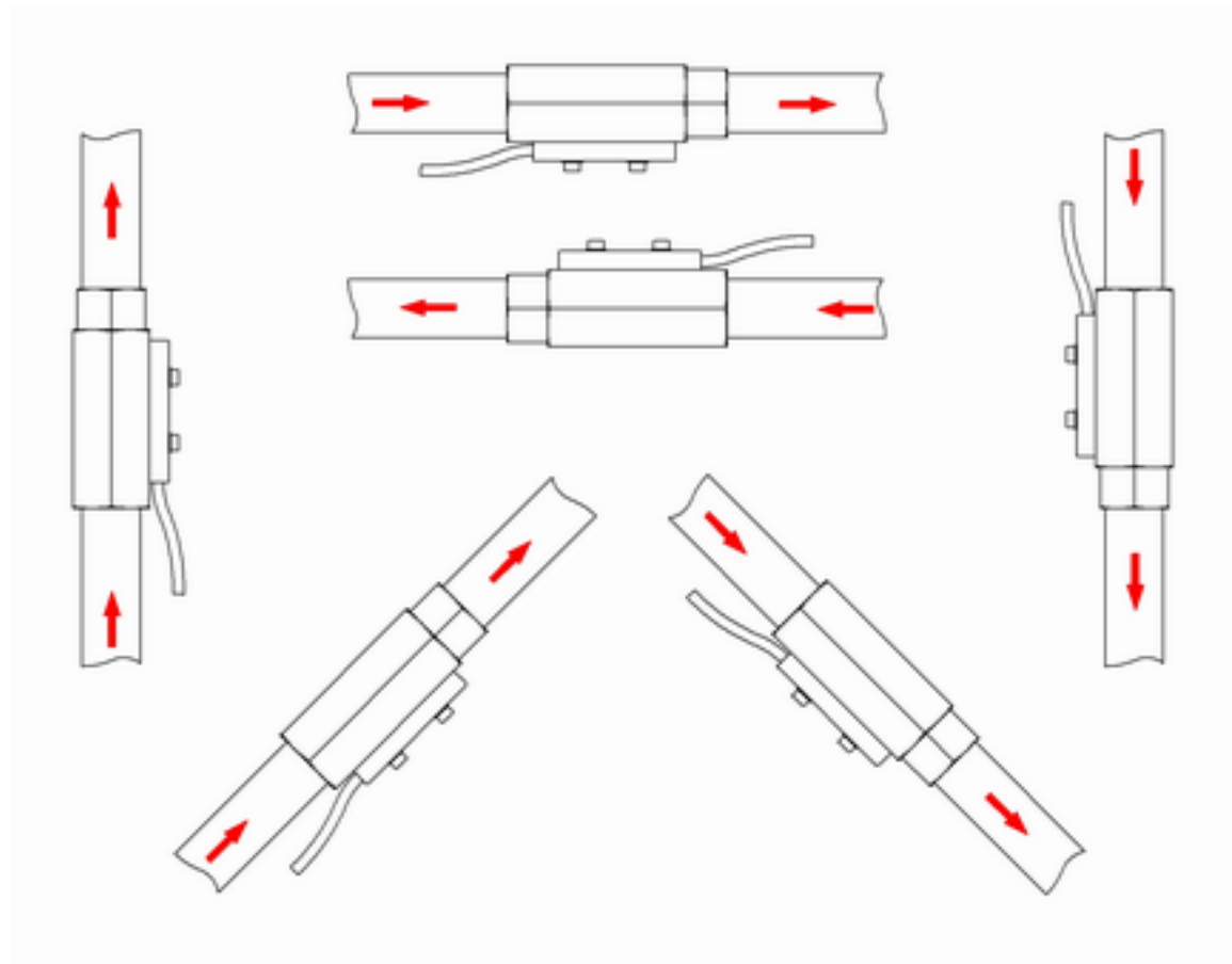
Fig. 5: Installation position/direction of flow
