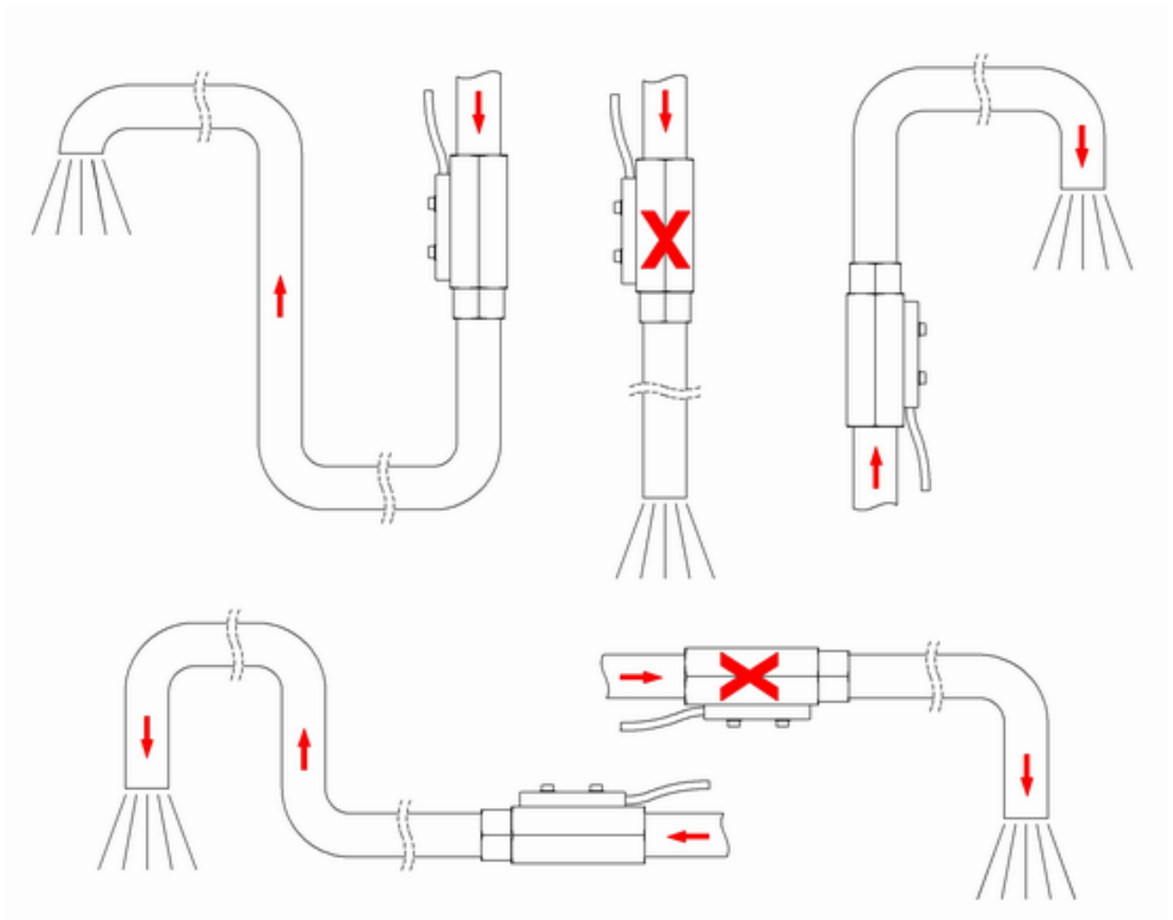
Fig. 7: Unimpeded outlet
