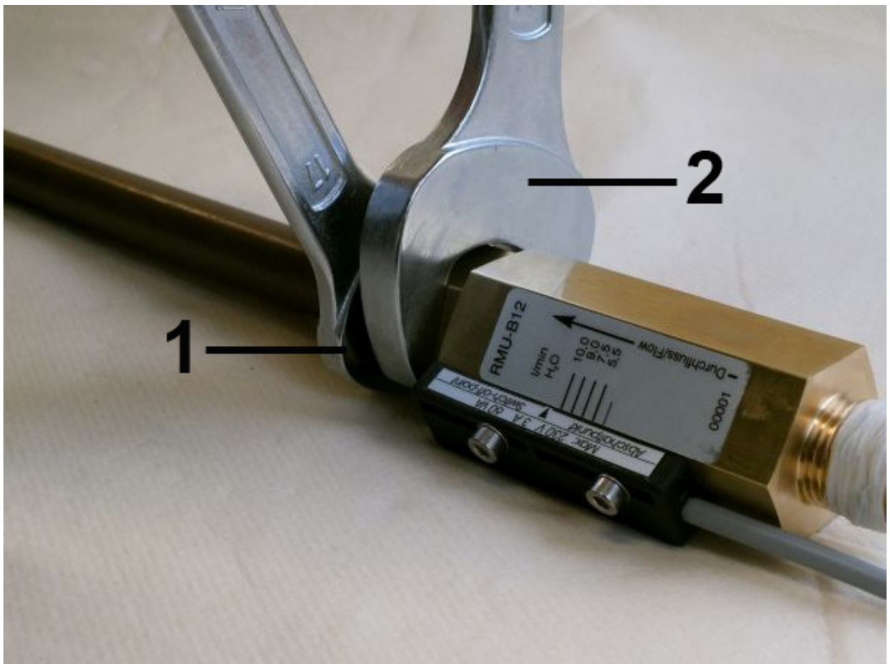
Fig. 15: Screw in the device (outlet)
