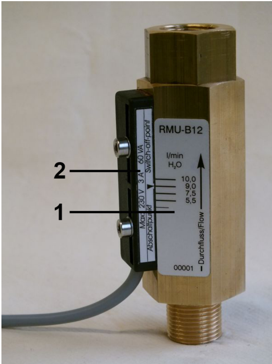
Fig. 1: RMU-B flow monitor
