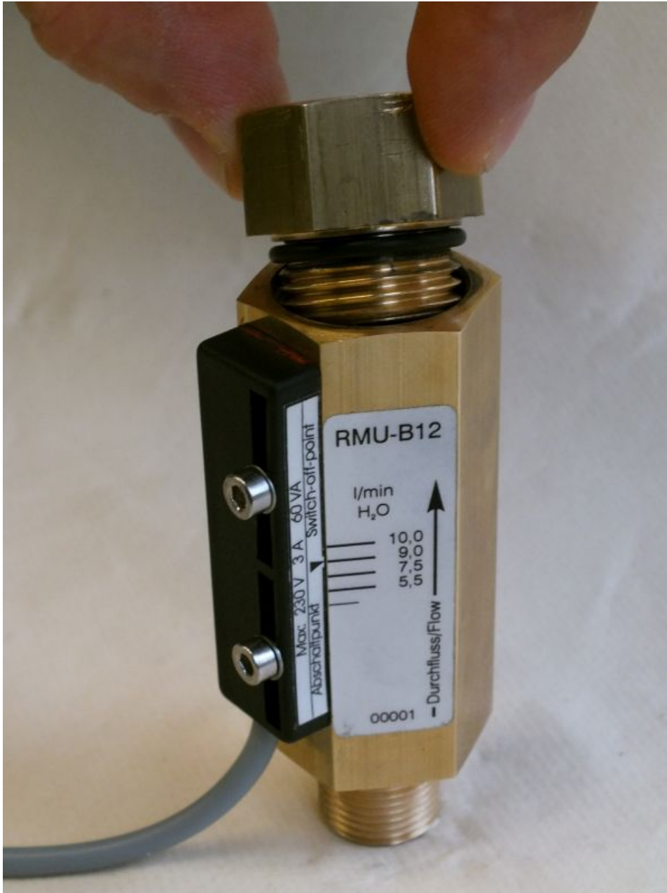
Fig. 34: Insert process connection (outlet)
