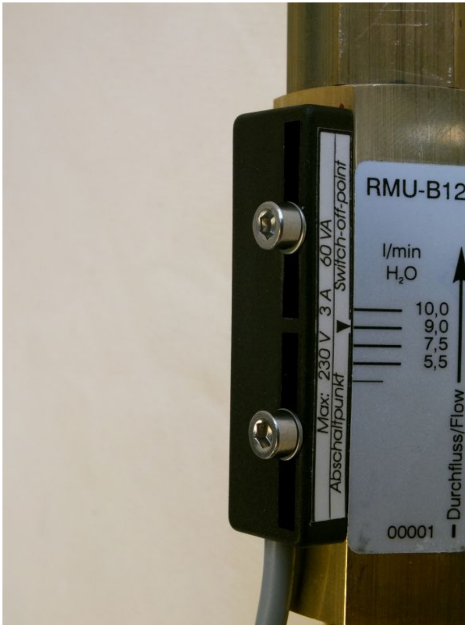
Fig. 4: Switch point adjustment scale
