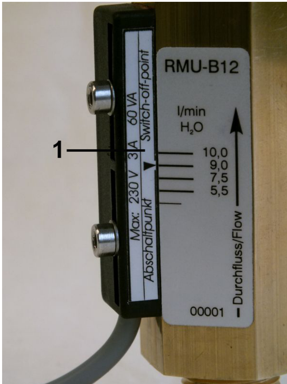
Fig. 3: Switch contact with connection cable
