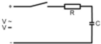
Fig. 16: Protective measure against capacitive loads
