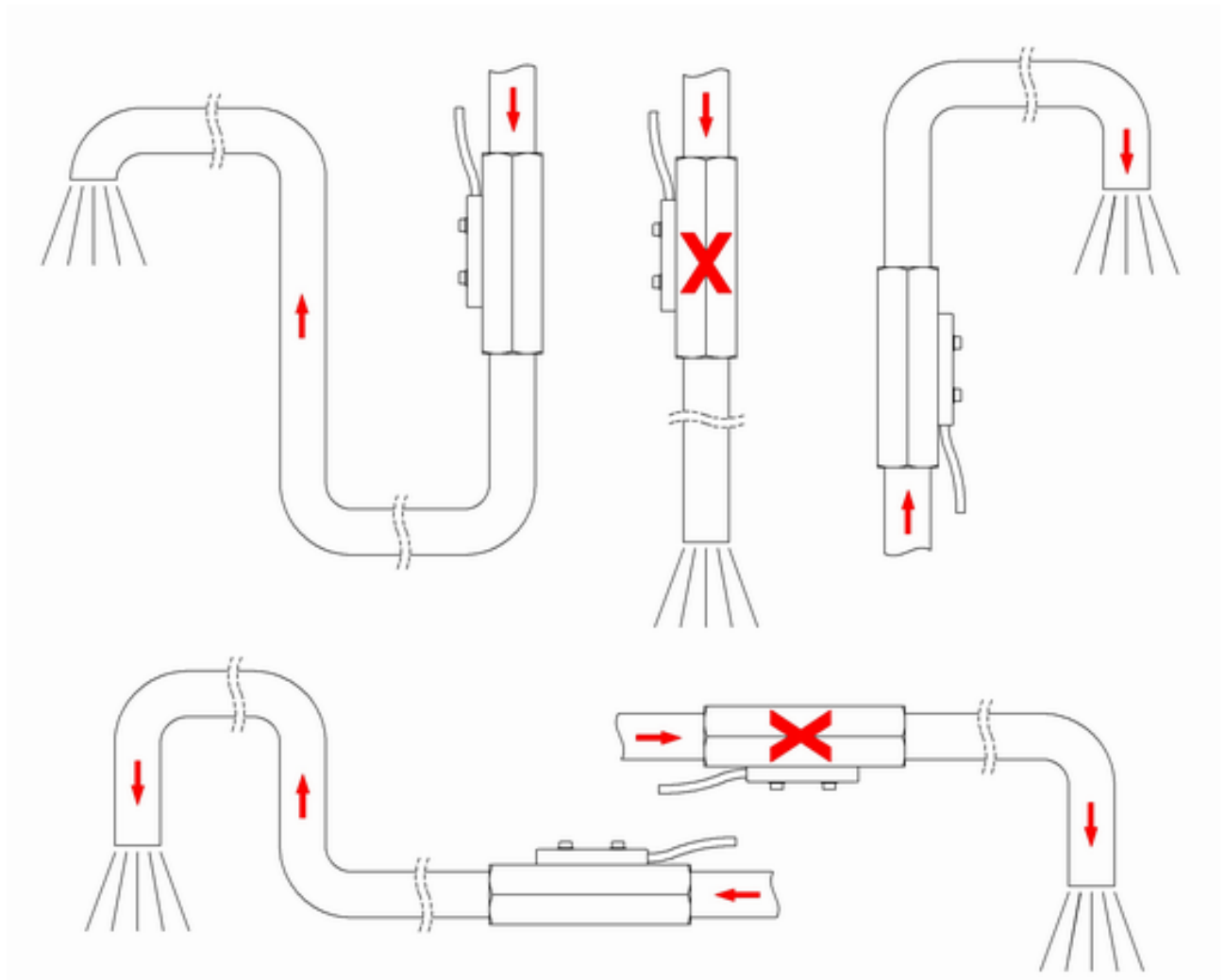
Fig. 7: Unimpeded outlet
