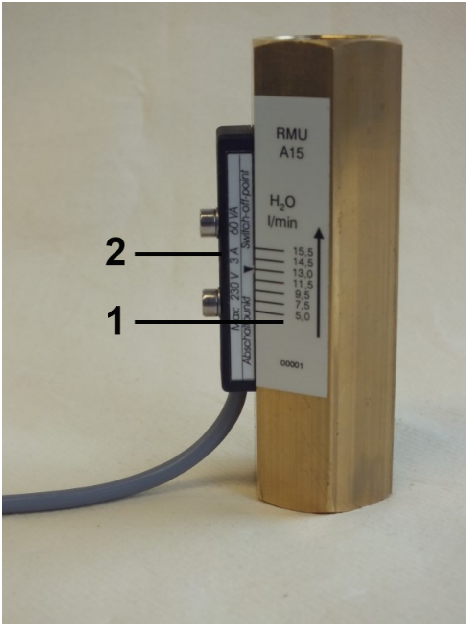
Fig. 1: RMU-A flow monitor
