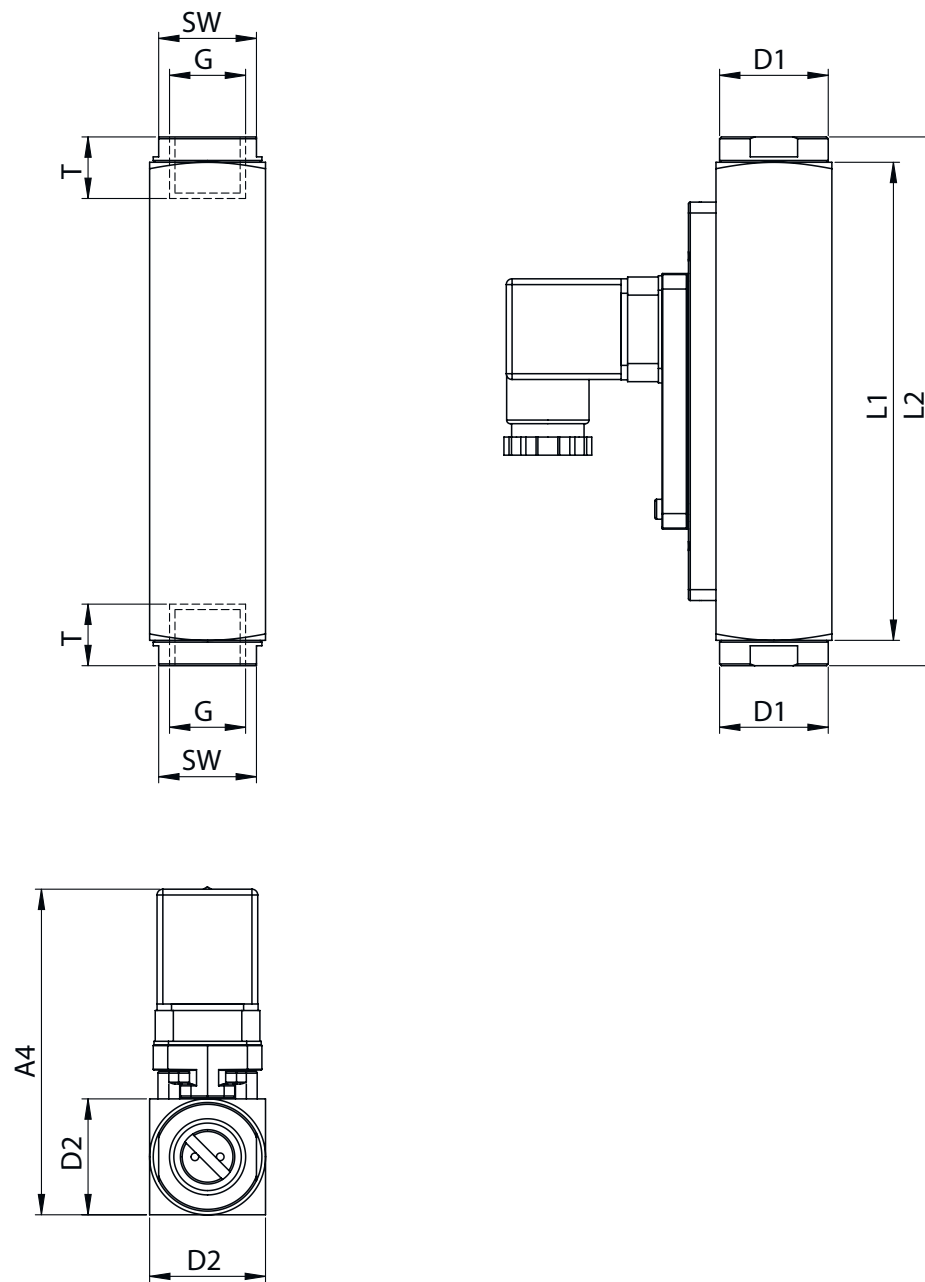
Fig. 68: TZ_DWM-18_SG-30
