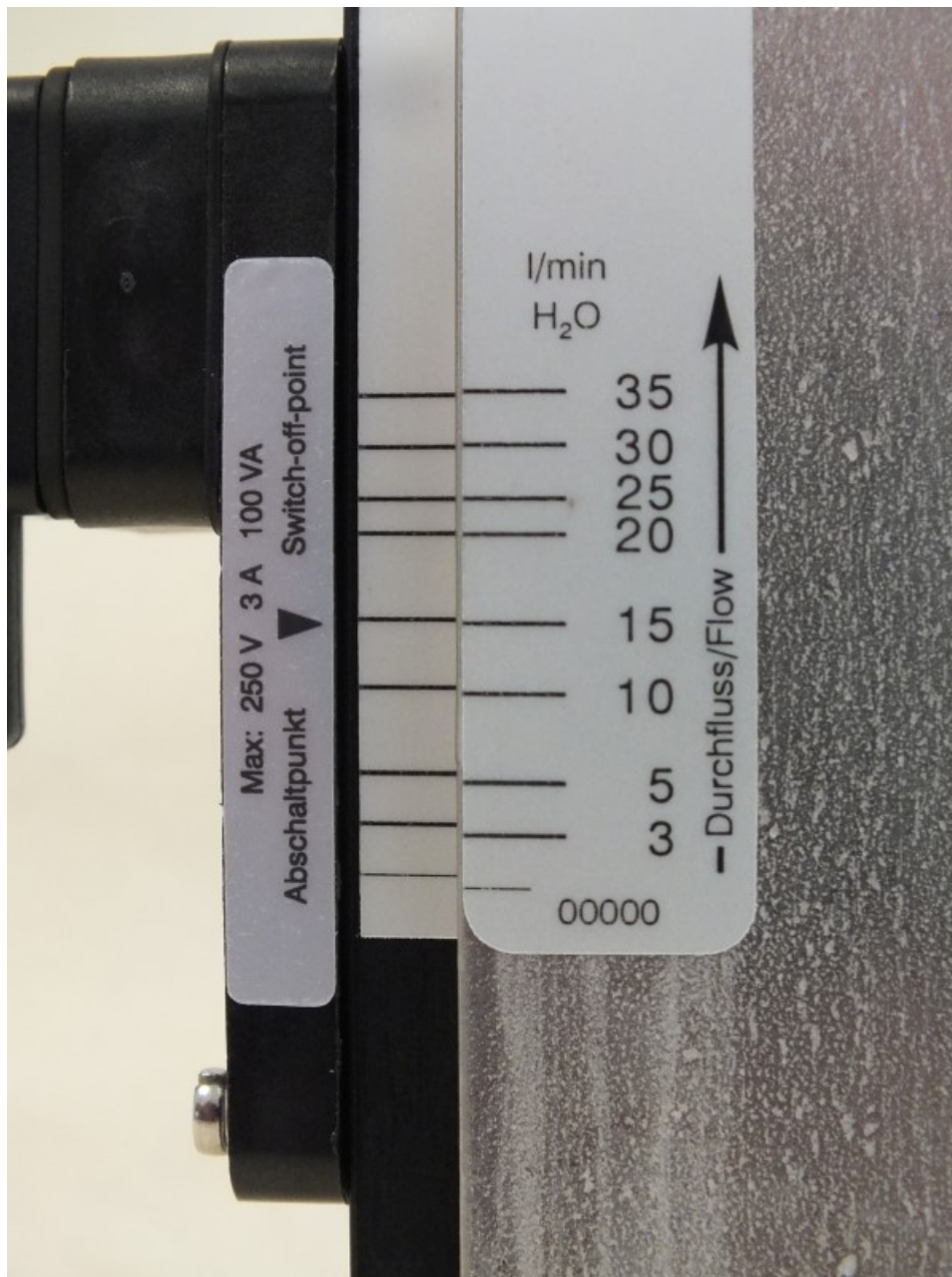
Fig. 4: DWM switch point adjustment scale
