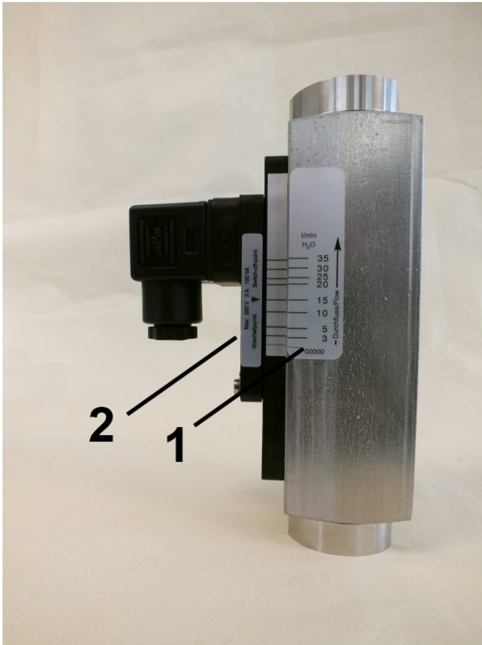
Fig. 1: DWM flow monitor
