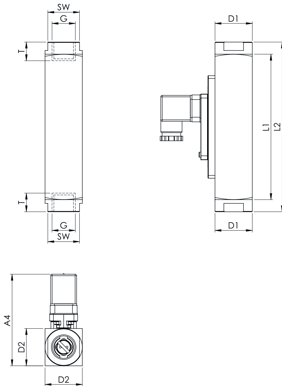
Fig. 69: TZ_DWM-50_SG-30
