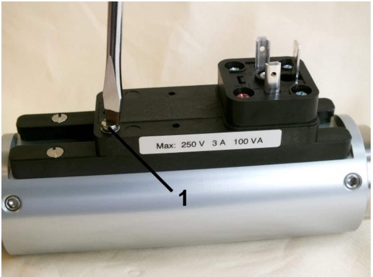
Fig. 65: Loosen set screws
