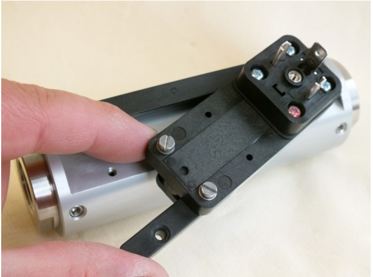
Fig. 67: Rotate guide rail to the side
