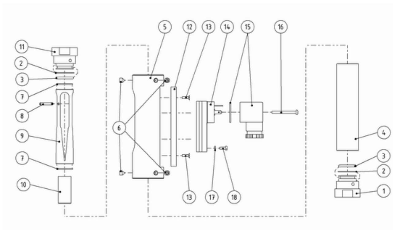
Fig. 74: Replacement parts drawing
