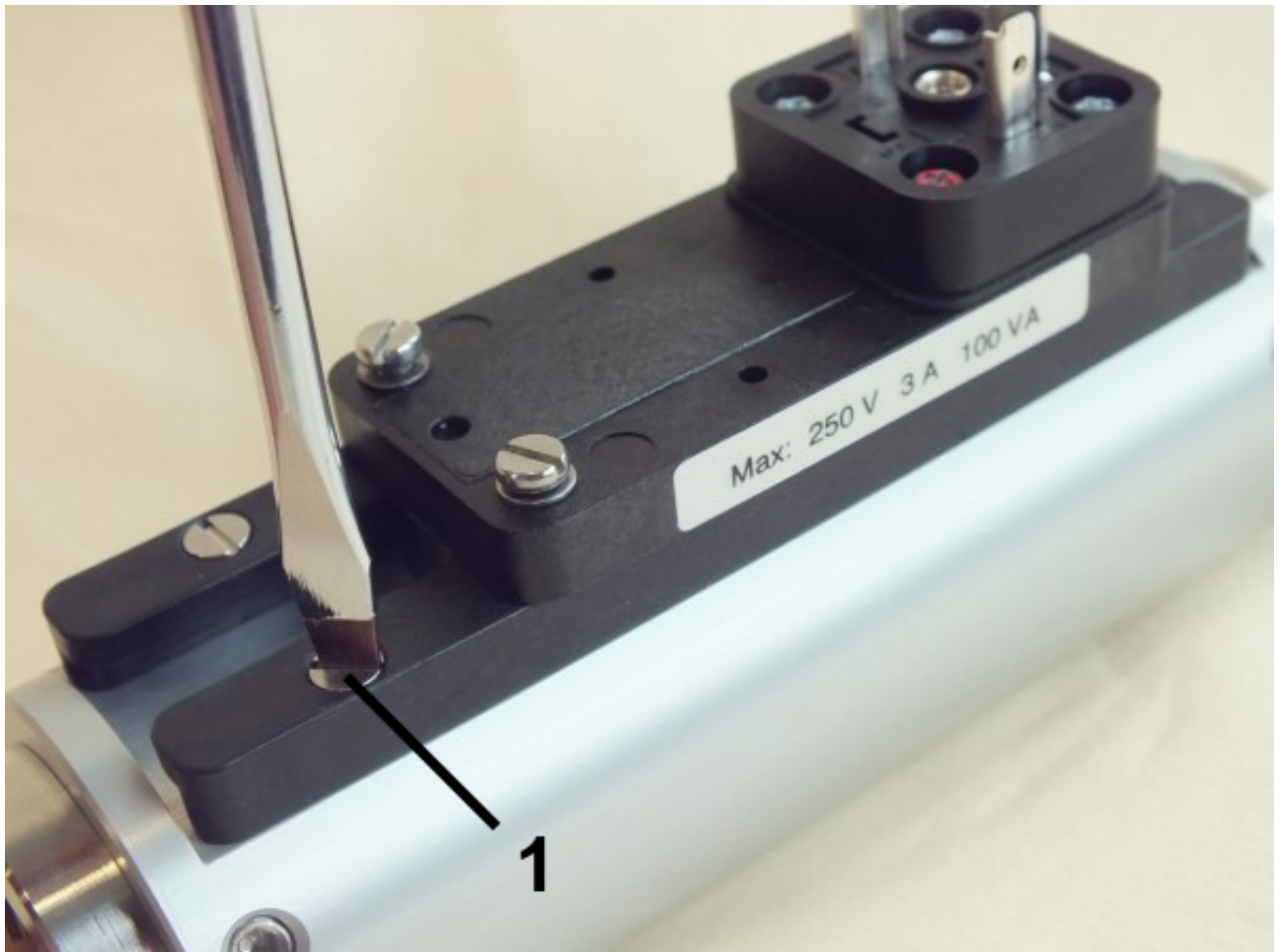
Fig. 66: Release the guide rail
