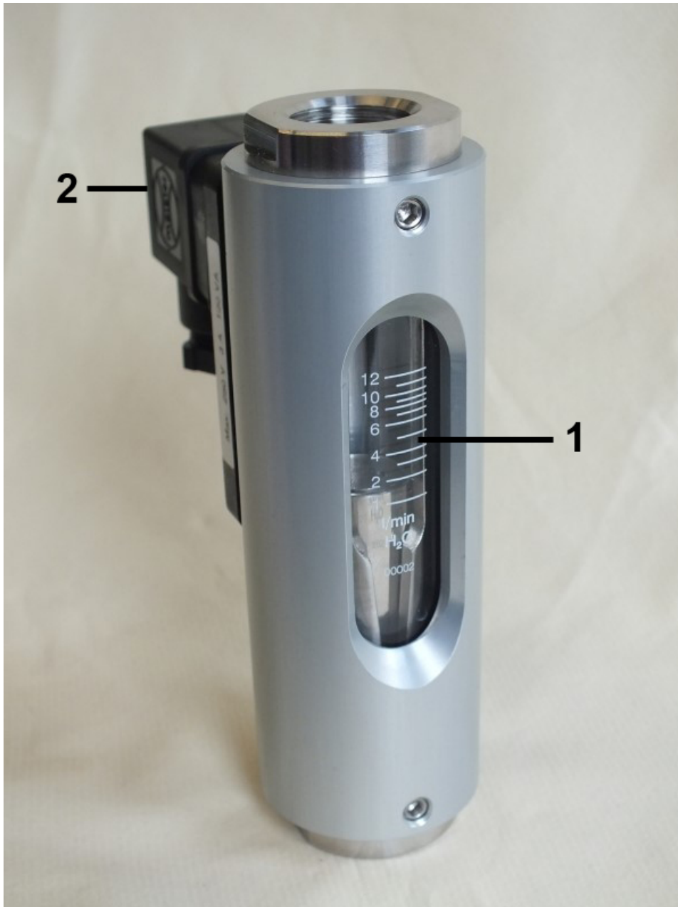
Fig. 1: DWG flow monitor
