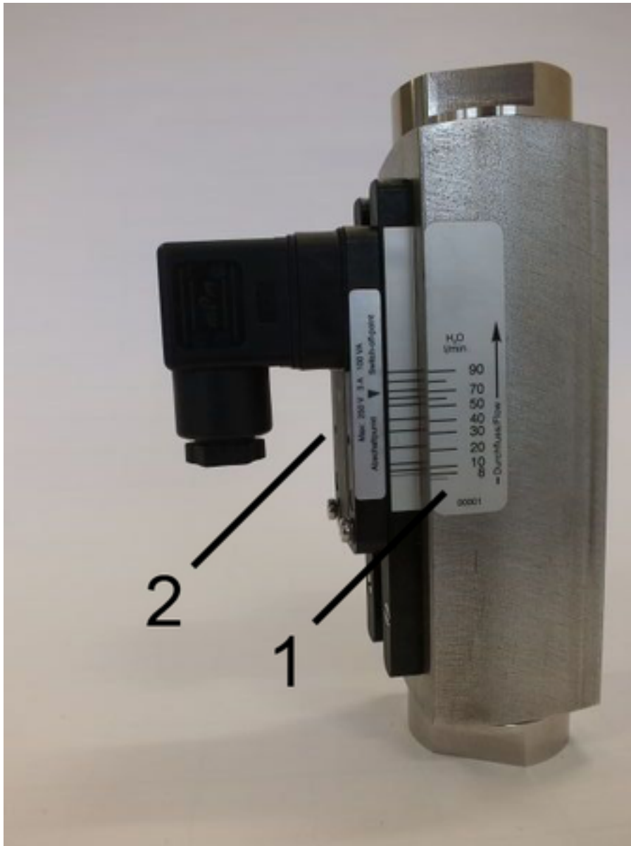
Fig. 1: DUM flow monitor
