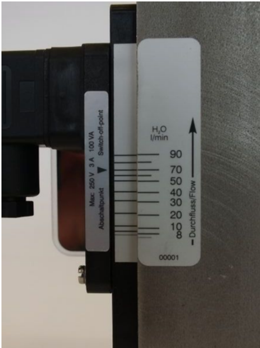
Fig. 4: DUM switch point adjustment scale
