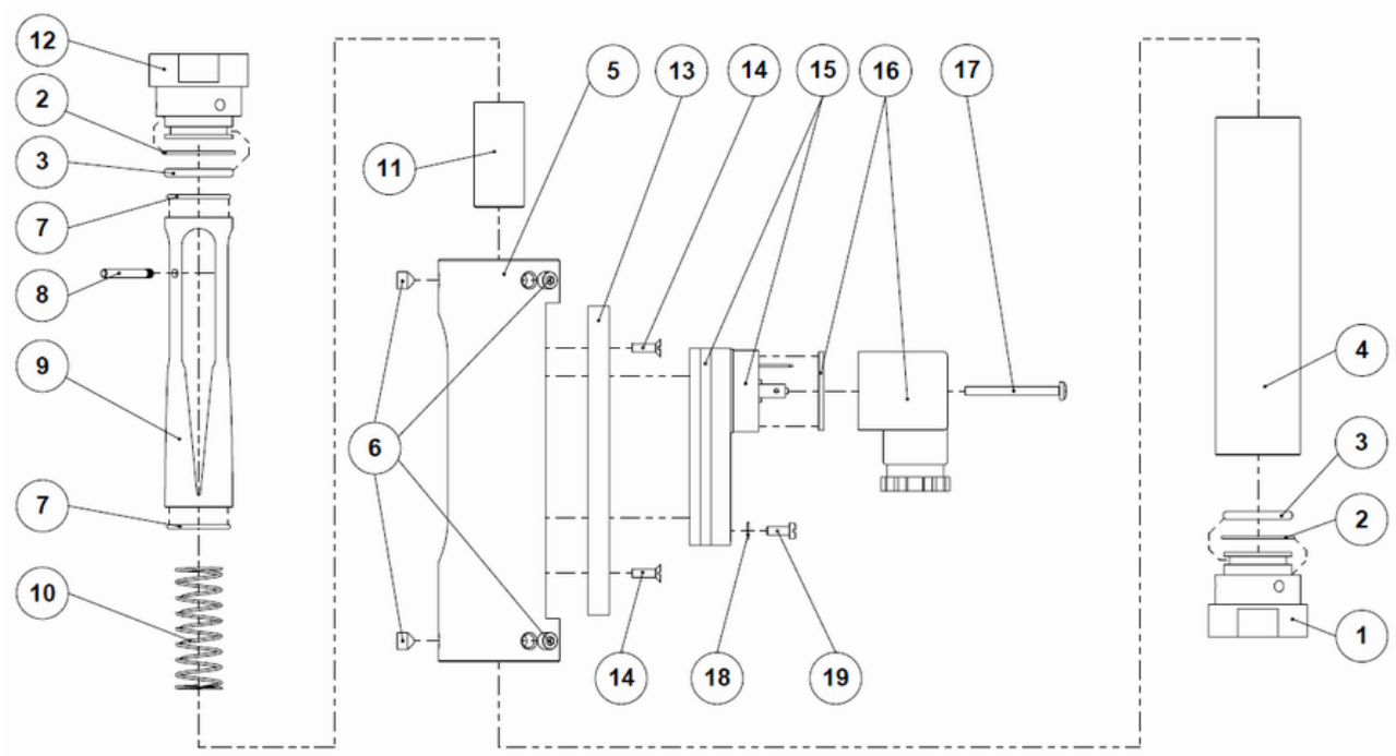
Fig. 76: Replacement parts drawing
