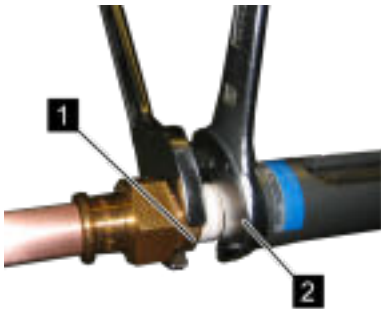
Fig. 12: Screw in the device
