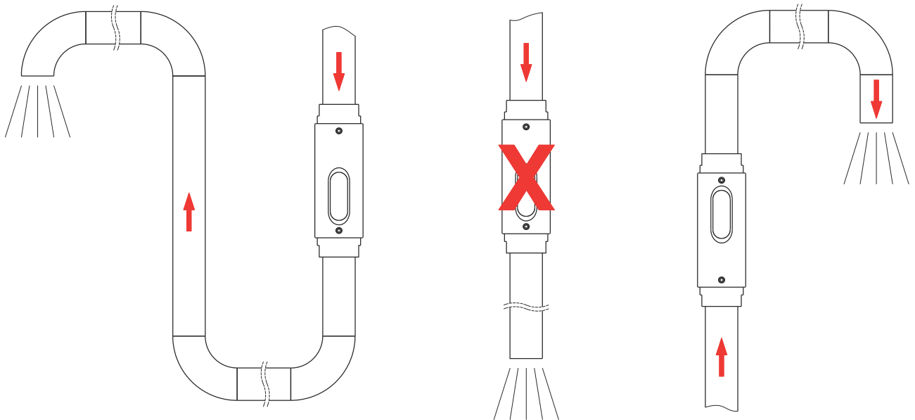
Fig. 7: Unimpeded outlet
