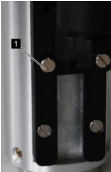
Fig. 39: Loosen set screws
