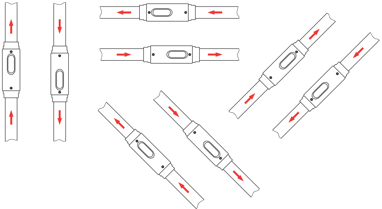
Fig. 5: Installation position/direction of flow
