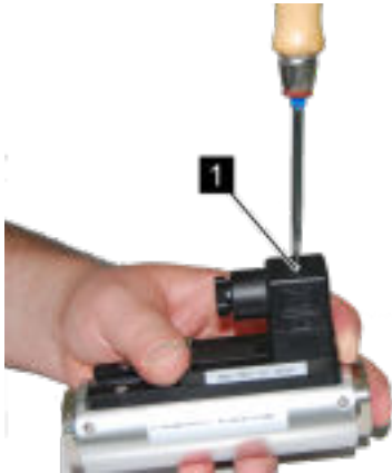
Fig. 64: Loosen female socket
