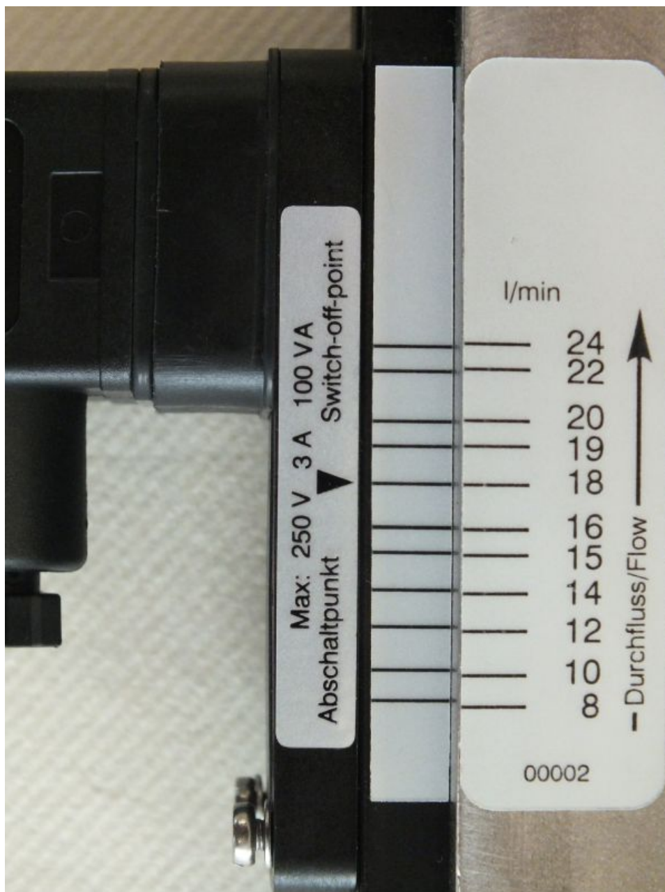
Fig. 4: Switch point adjustment scale DKME/A-1
