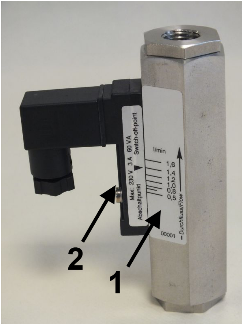
Fig. 1: DKM-2 flow monitor
