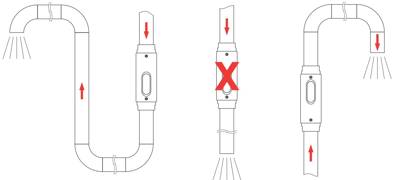
Fig. 7: Unimpeded outlet
