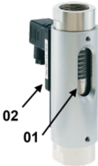
Fig. 1: DKG-1 flow monitor
