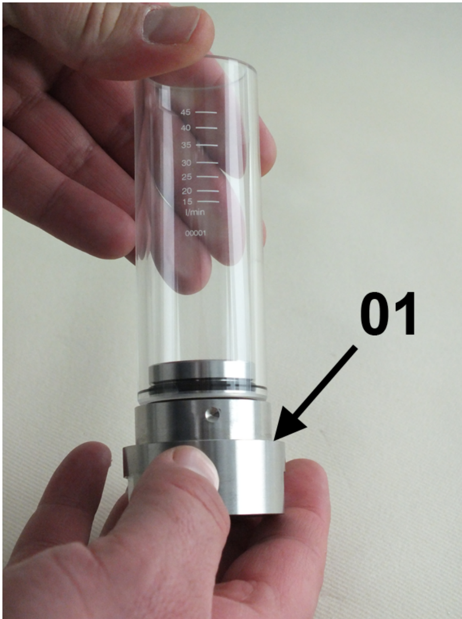
Fig. 50: Process connection (inlet) in sight glass
