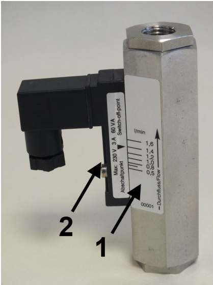
Fig. 1: DKM-2 flow monitor
