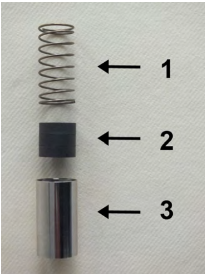
Fig. 42: Spring, magnets and float
