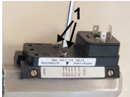
Fig. 58: Loosen set screws
