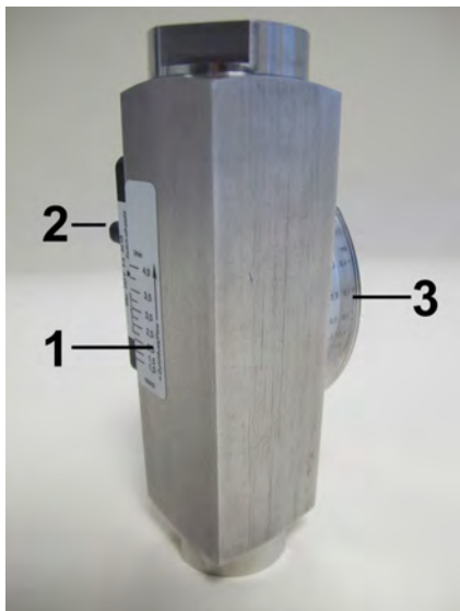
Fig. 1: DWM/A flow monitor
