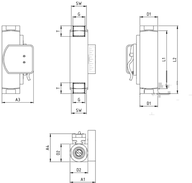
Fig. 3: Type DWM/A-35 through DWM/A-50 (G \frac{3}{4} " )
