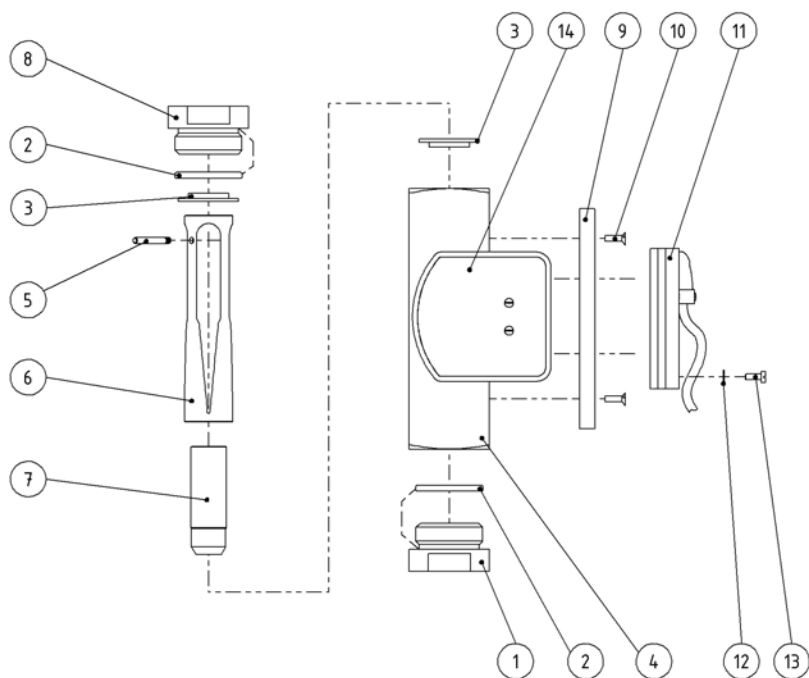
Fig. 6: Type DWM/A-L18 through DWM/A-L50 (G \frac{3}{4} " )
