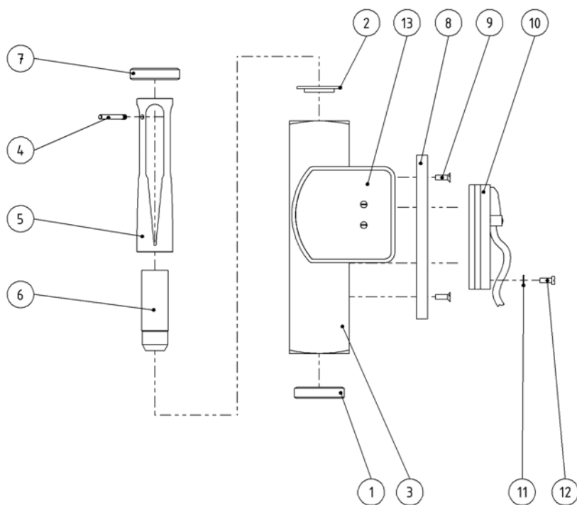
Fig. 7: Type DWM/A-L50 through DWM/A-L100 (G1")
