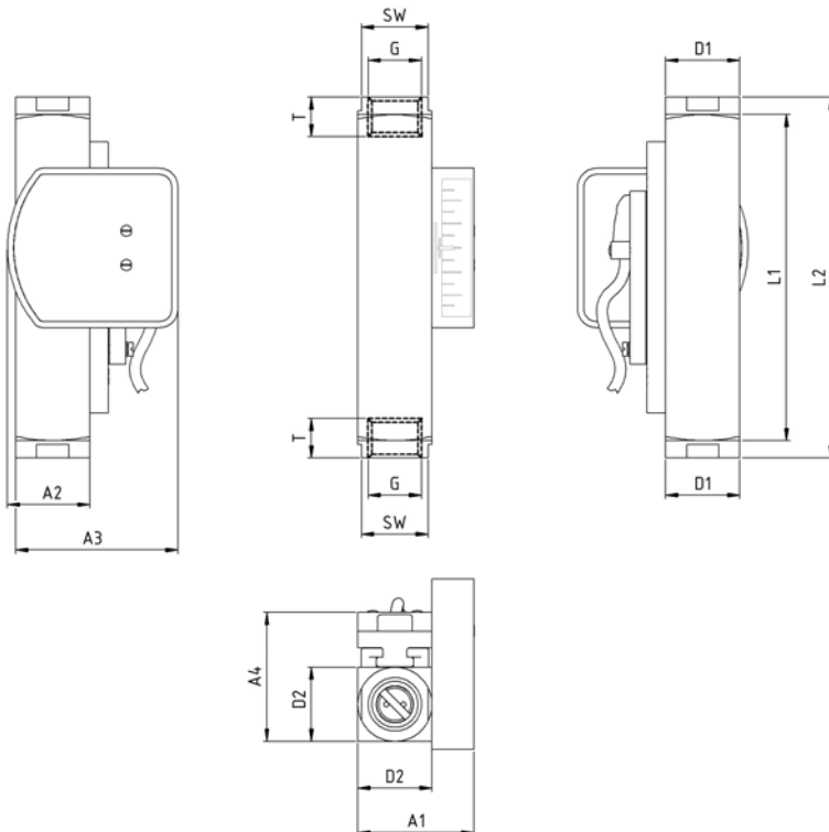
Fig. 2: Type DWM/A-L1,5 through DWM/A-L18
