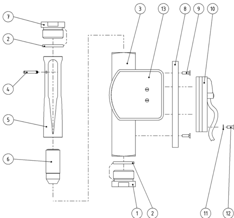
Fig. 5: Type DWM/A-L1,5 through DWM/A-L18
