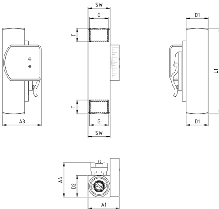
Fig. 4: DWM/A-L50 through DWM/A-L100 (G1")
