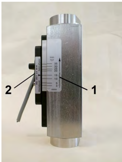
Fig. 1: DWM flow monitor
