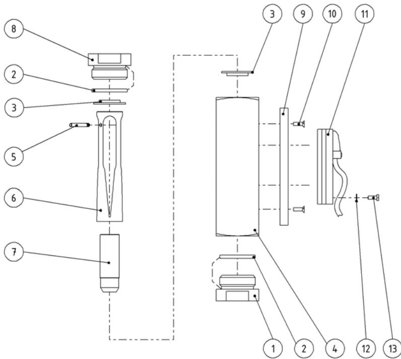
Fig. 6: Type DWM-L18 through DWM-L50 (G3/4")
