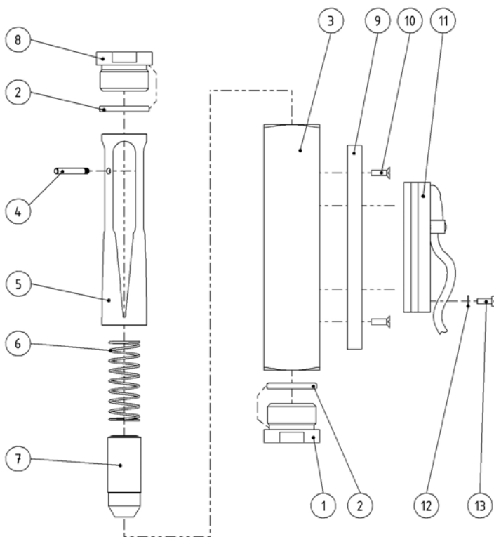
Fig. 5: Type DUM-55 ATEX
