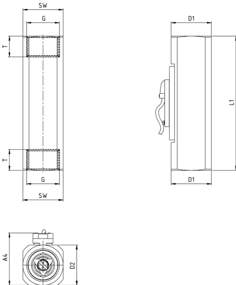
Fig. 4: Type DUM-220 ATEX and DUM-250 ATEX
