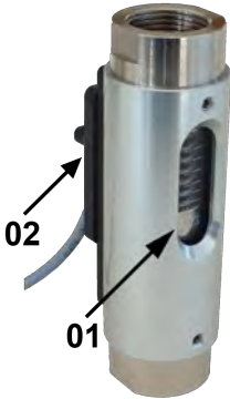
Fig. 1: Flow monitor DKG-1
