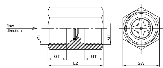
Fig. 4: Dimension sheet BA
