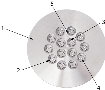
Fig. 2: Overview Flow limiter
