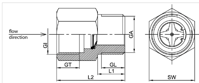
Fig. 5: Dimension sheet BB
