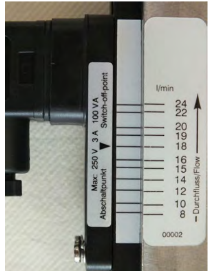
Fig. 4: Switch point adjustment scale DKM-1
