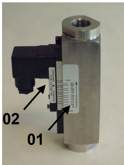
Fig. 1: DKM-1 flow monitor
