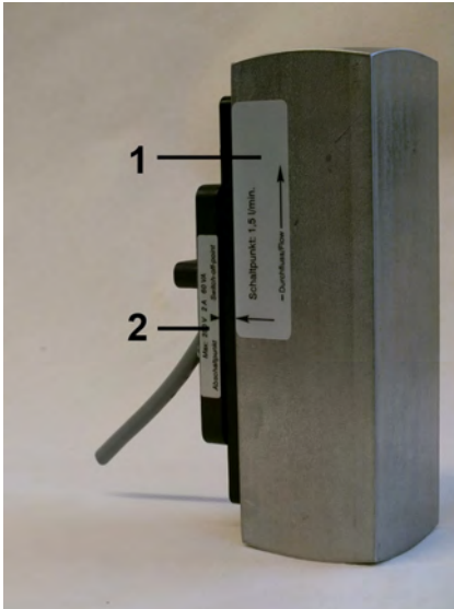
Fig. 1: Flow monitor RVM/UM
