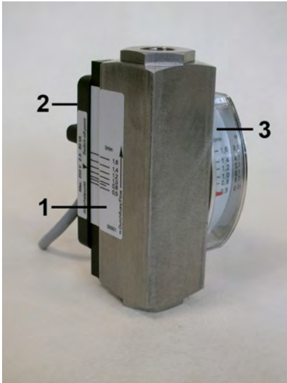
Fig. 1: DKM/A-2 30x70 flow monitor
