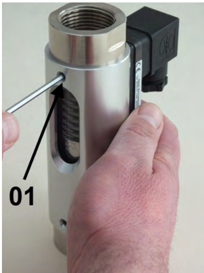
Fig. 37: Remove the process connection (outlet)
