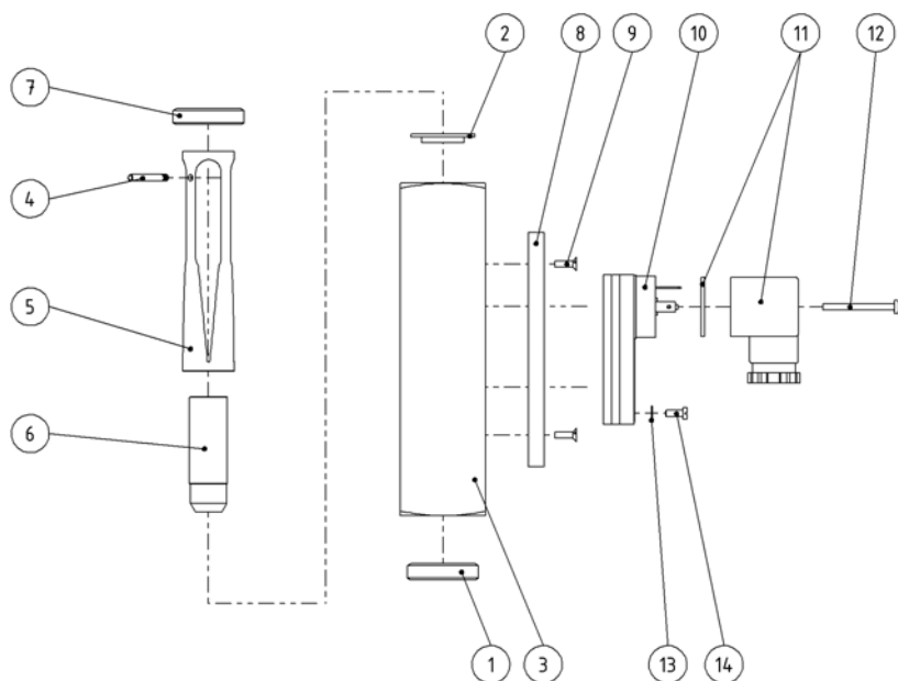
Fig. 67: Type DWM-L50 through DWM-L100 (G1")
