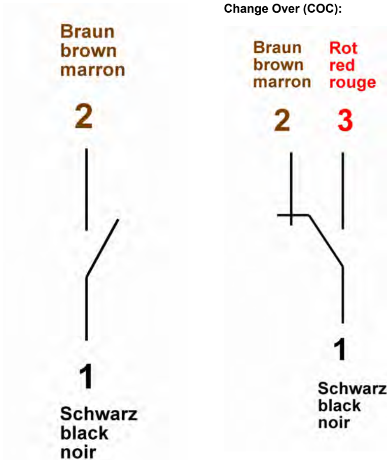
Fig. 20: Switch position under no-flow condition
