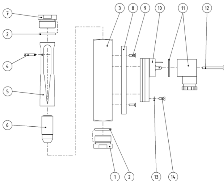
Fig. 65: Type DWM-L1,5 through DWM-L18
