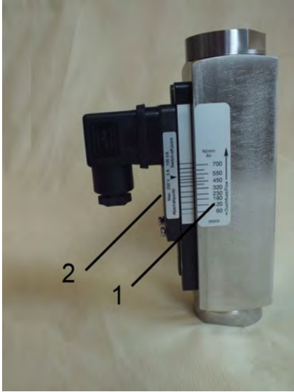
Fig. 1: DWM-L flow monitor
