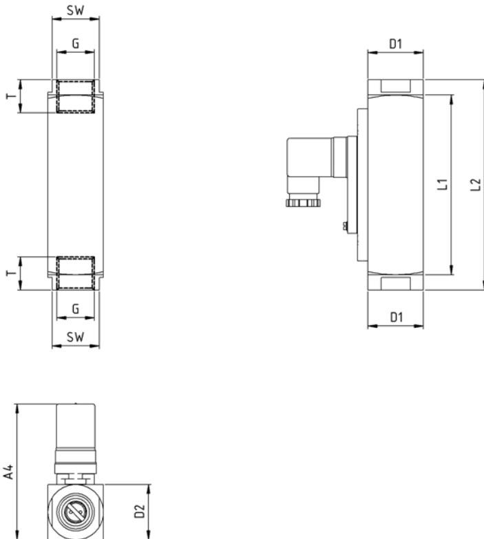
Fig. 63: Type DWM-L50 (G \frac{3}{4} " )
