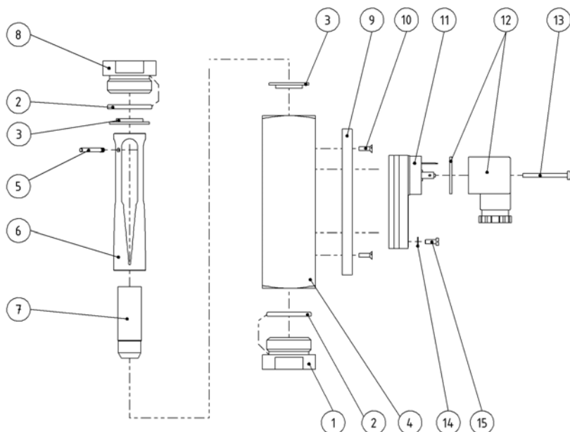
Fig. 66: Type DWM-L50 (G3/4")
