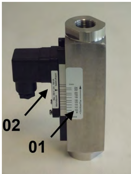
Fig. 1: DKME-1 flow monitor
