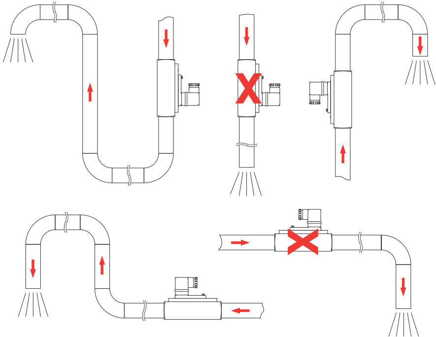
Fig. 7: Unimpeded outlet
